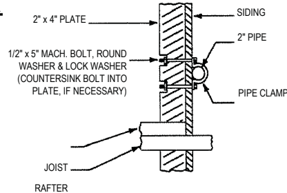
DETAIL "A" METHOD OF ATTACHING 2" PIPE TO BUILDING PLATE
