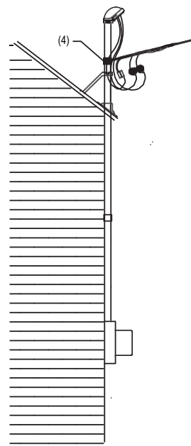
FIGURE 2: ATTACHMENT ON SERVICE RISER
